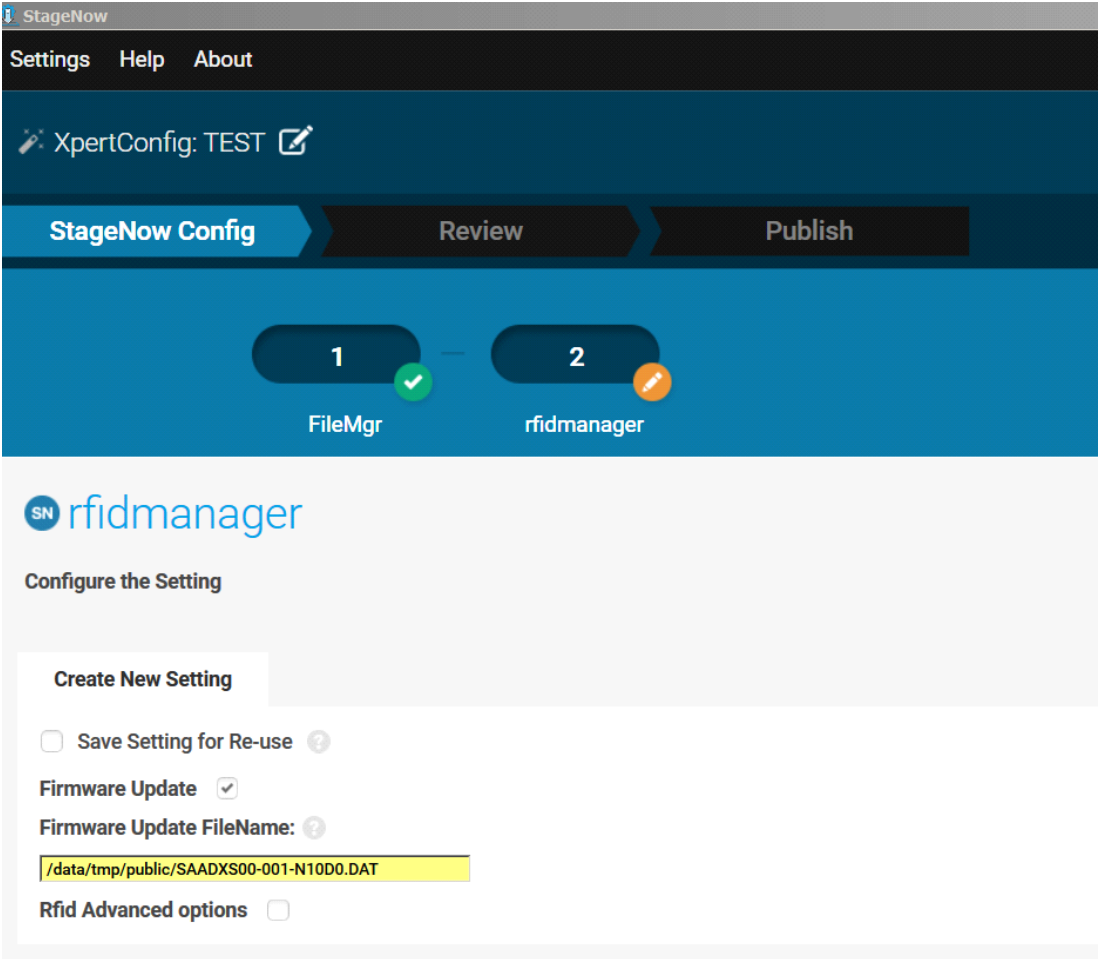
Figure 56 Create Firmware Update-RfidManager Configuration
