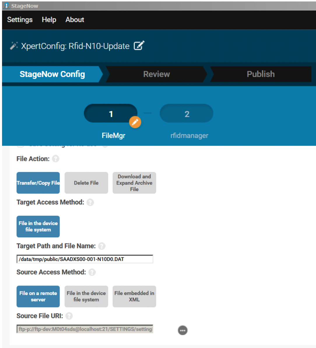
Figure 55 Create Firmware Update-FileMgr Configuration
