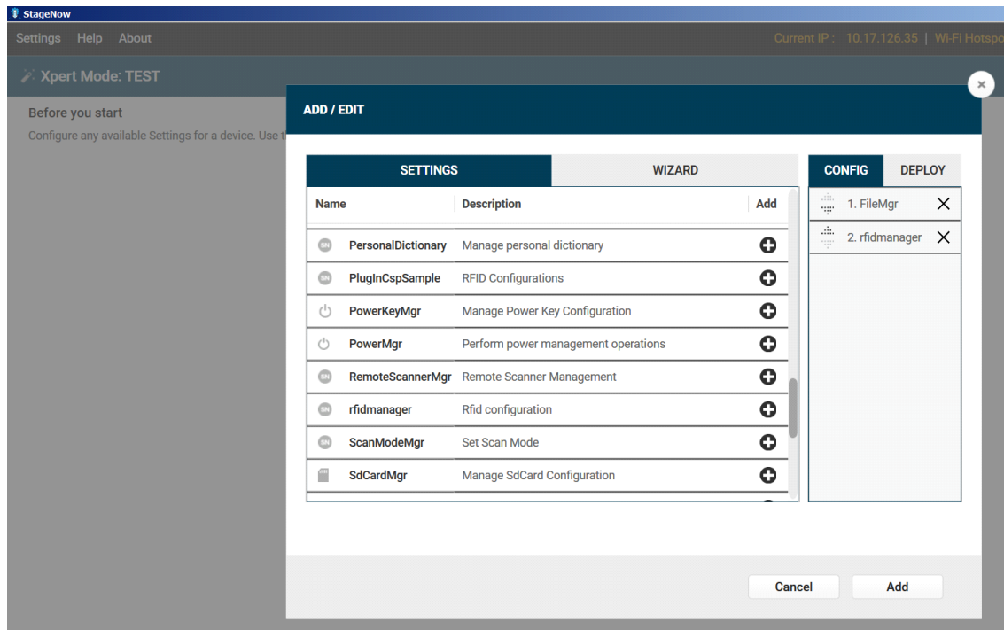
Figure 54 Create Firmware Update-Add Applications
